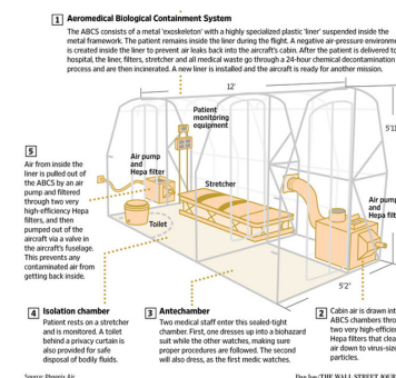
Figure 5: ABCS system (Source Phoenix Air)
